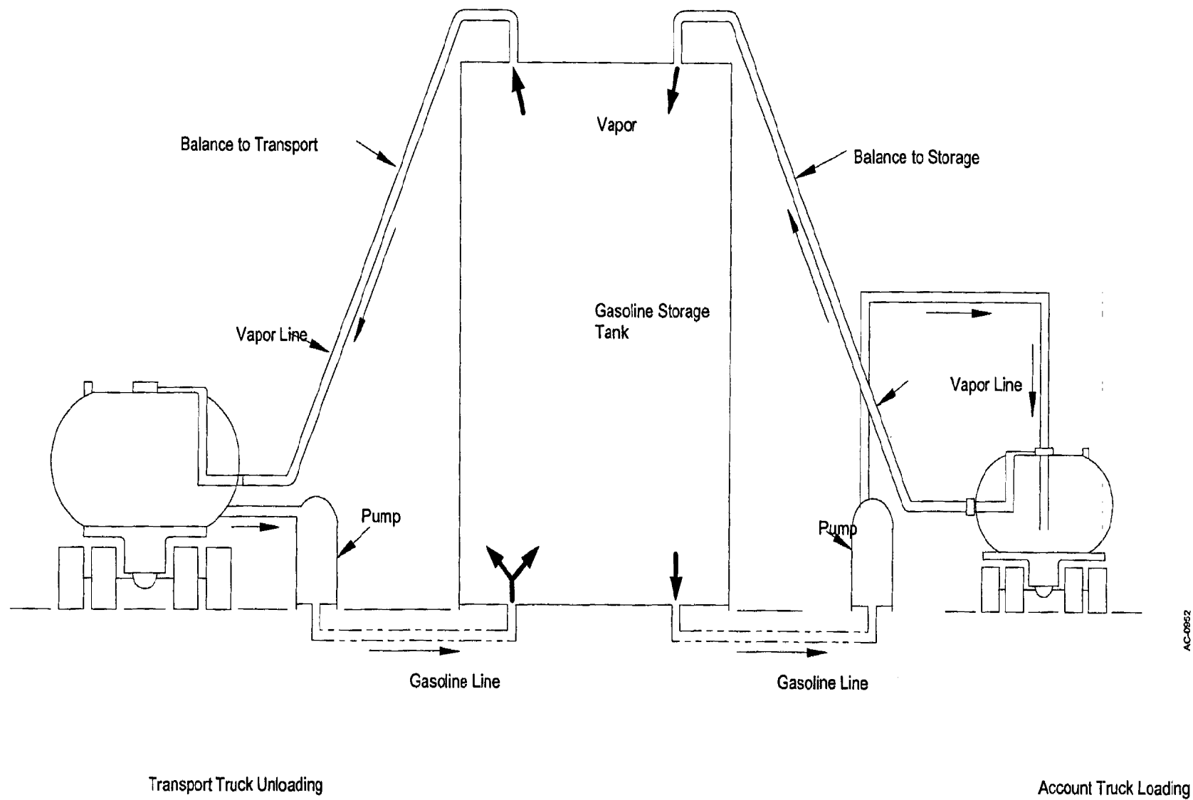
Figure 6-4. Bulk Plant Vapor Balance System (Stage I)
