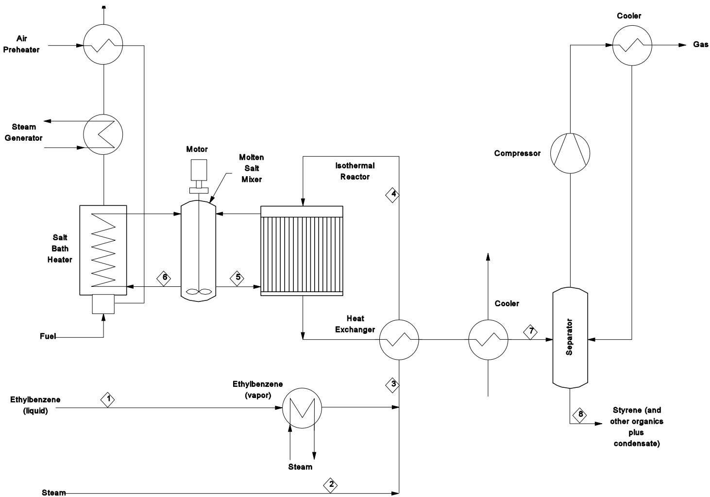
Figure 5-4. Isothermal Processing of Styrene
