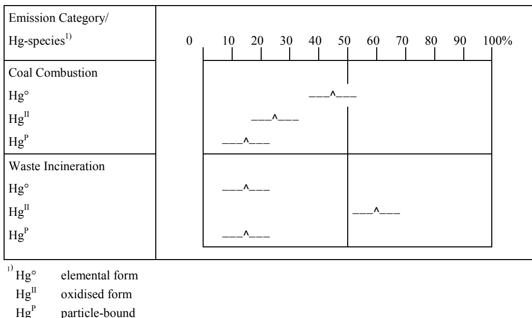
Figure 2: Contribution of various forms of mercury to the emissions from combustion source categories in Europe in 1987 (in % of total) /29/
